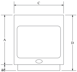
VFG 700 COAL GRATE
