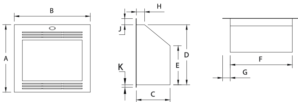
VFG 600 COAL GRATE
